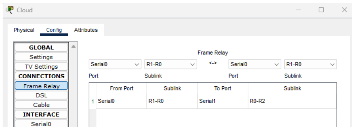
Figure 13.6 : Shows the link between Serial0 and Serial1 in Frame Relay
