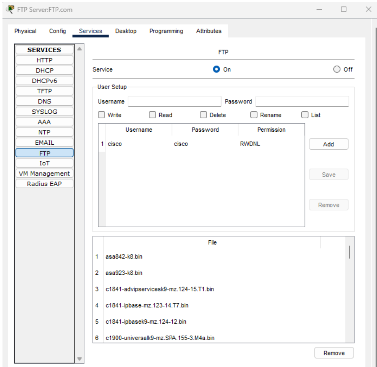
Figure 11.2. FTP Service Configuration
