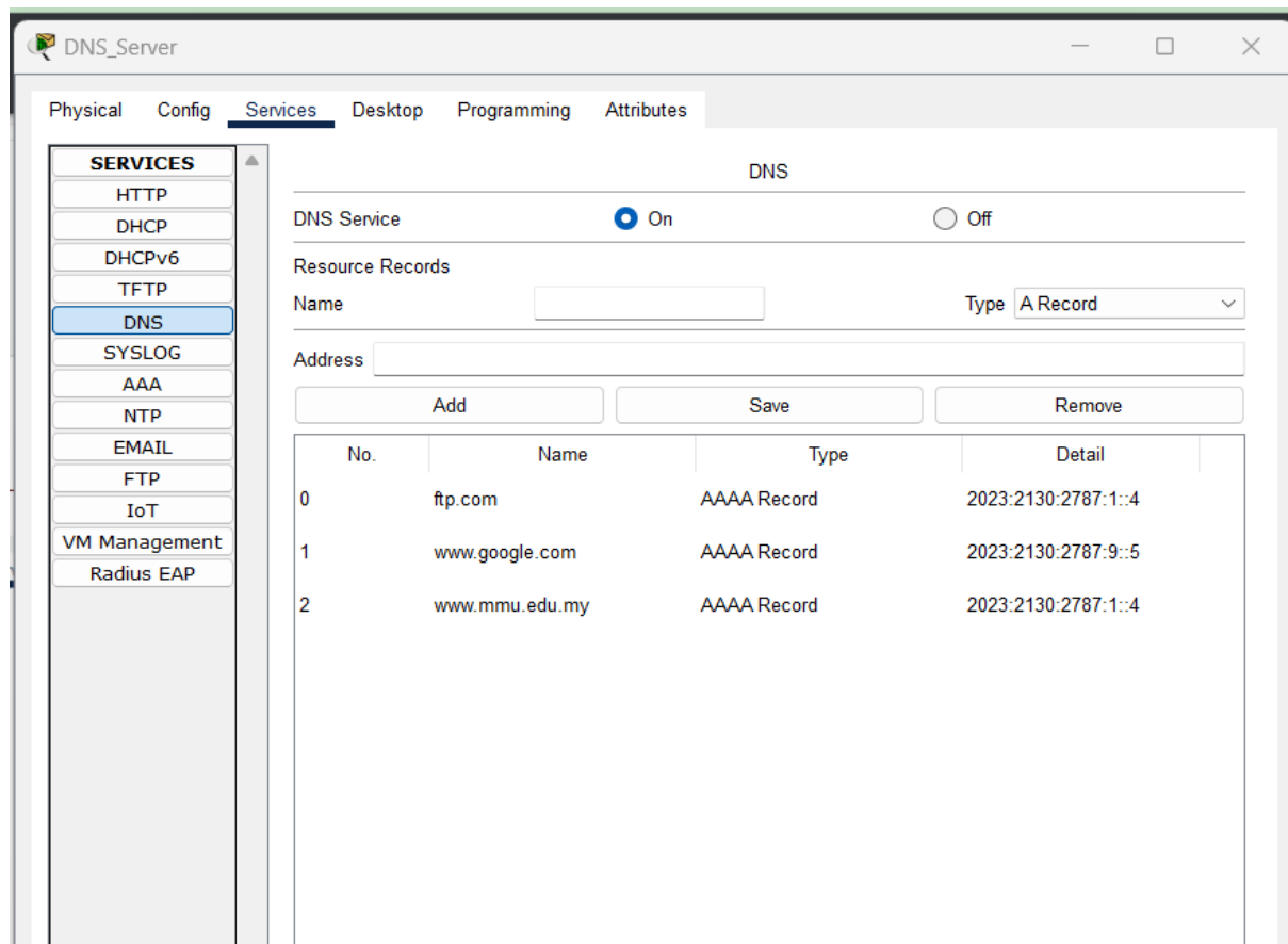
Figure 12.2. DNS services configuraion for DNS Server
