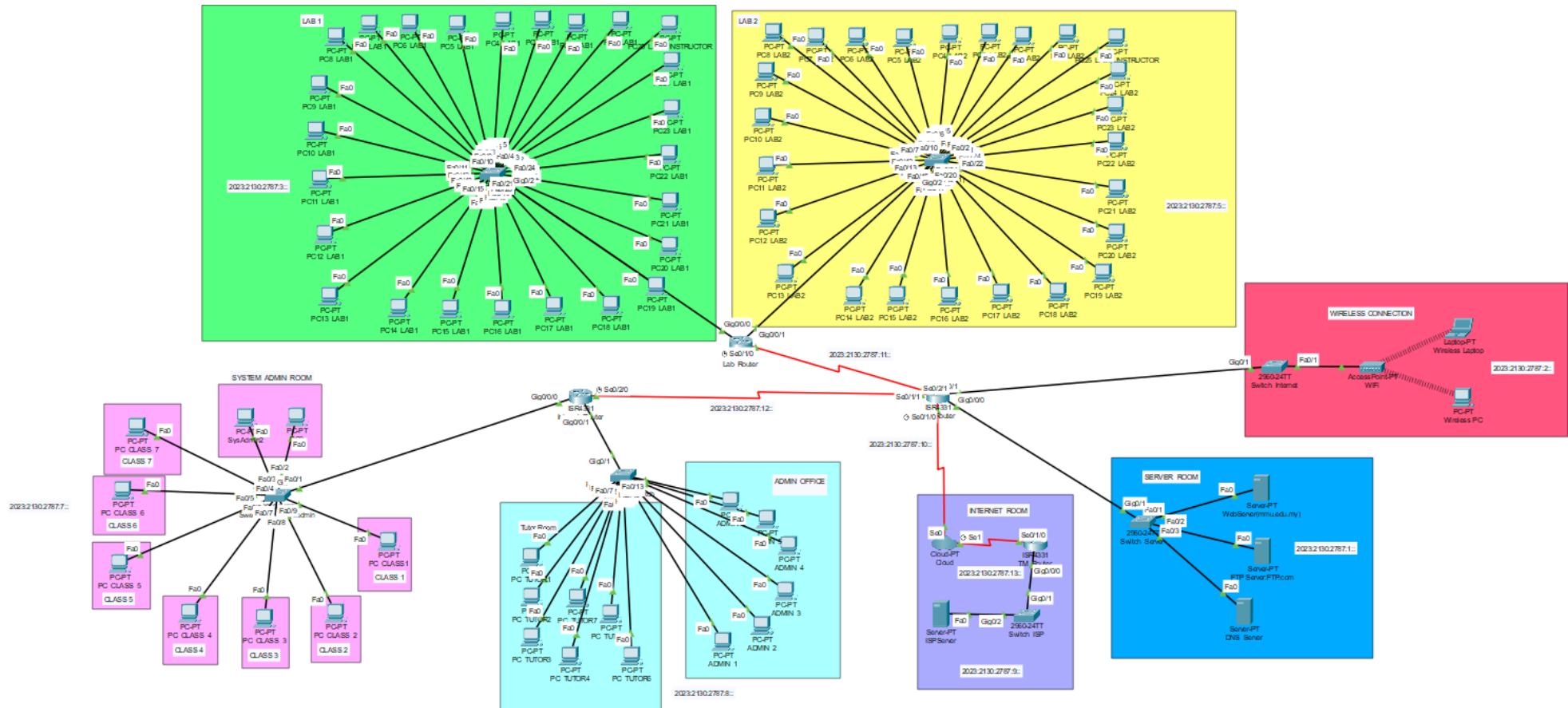
Figure 1- Logical Topology
