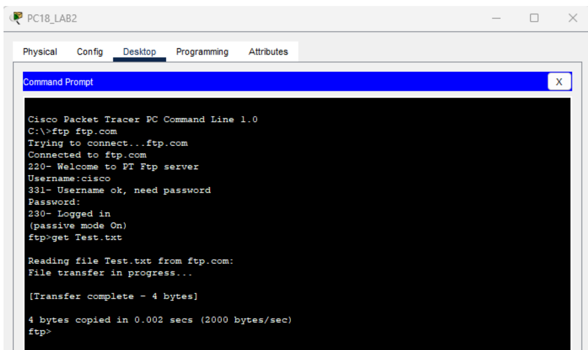
Figure 11.5 : Downloading Test.txt file to PC18_lab2
